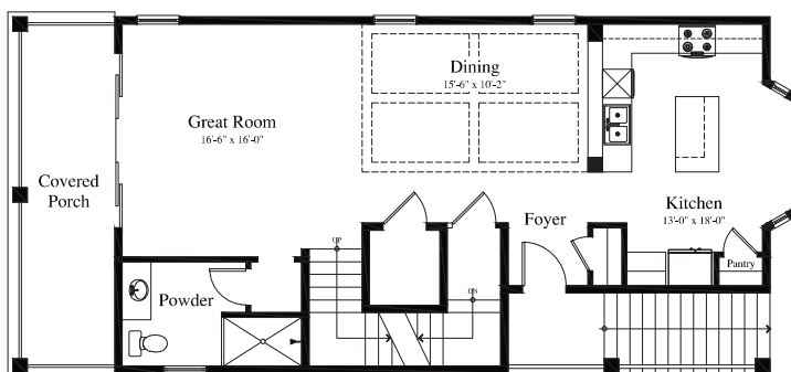
Main Level - 1022 sq. ft.
