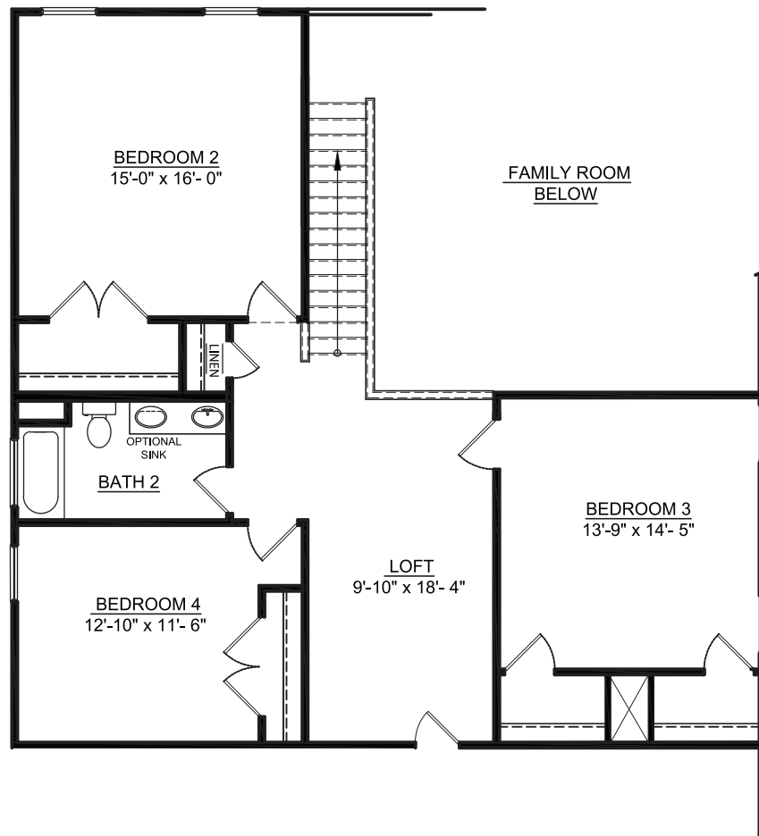
OPTIONAL SECOND FLOOR
