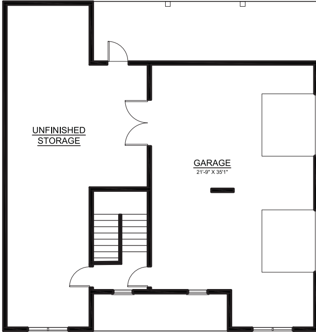
GARAGE LEVEL
