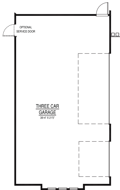
OPTIONAL THREE CAR GARAGE
