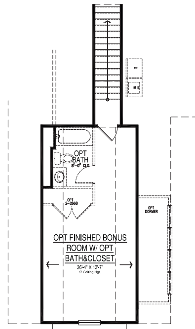
OPT FINISHED BONUS ROOM W/OPT BATH&CLOSET
