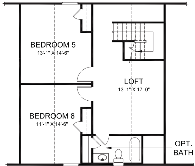
OPTIONAL THIRD FLOOR W/ OPTIONAL BEDROOMS & BATH
