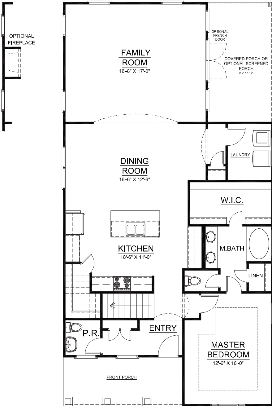
(OPTIONAL)FIRST FLOOR PLAN
