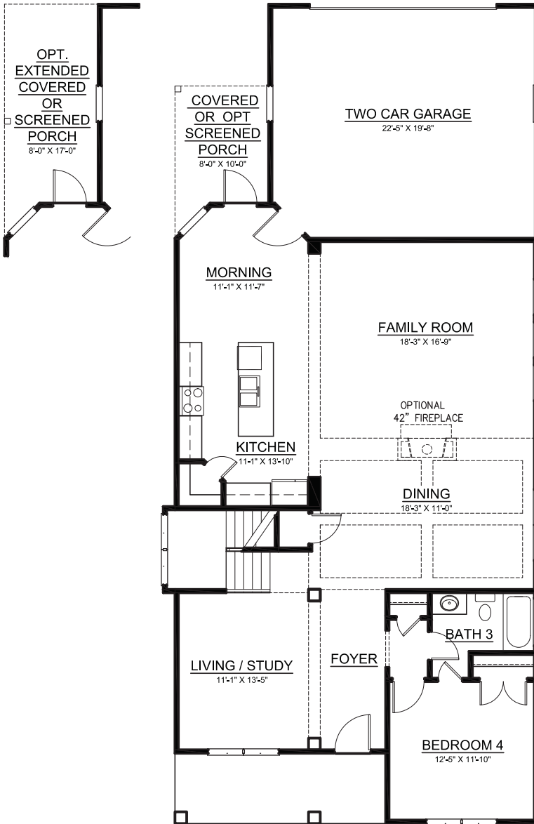
FIRST FLOOR PLAN 21' X 50'
