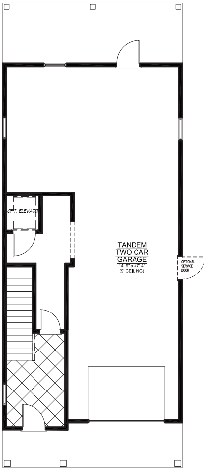
FIRST FLOOR PLAN "A" & "B" SCALE: 1/4" = 1'-0"
