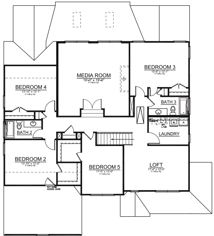
SECOND FLOOR PLAN 1874 SQ. FT.
